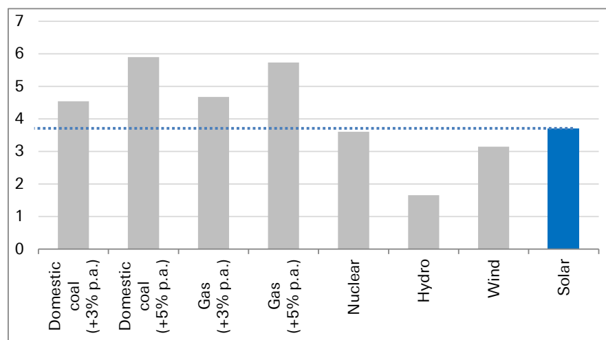
Figure 6: LCOE of energy sources in India highlights attractiveness of solar
